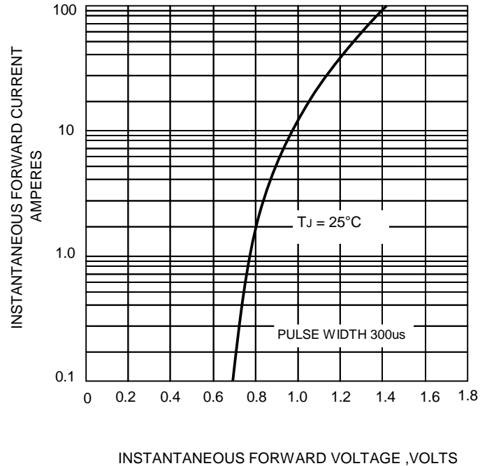
FIG.4-TYPICAL FORWARD CHARACTERISTICS
