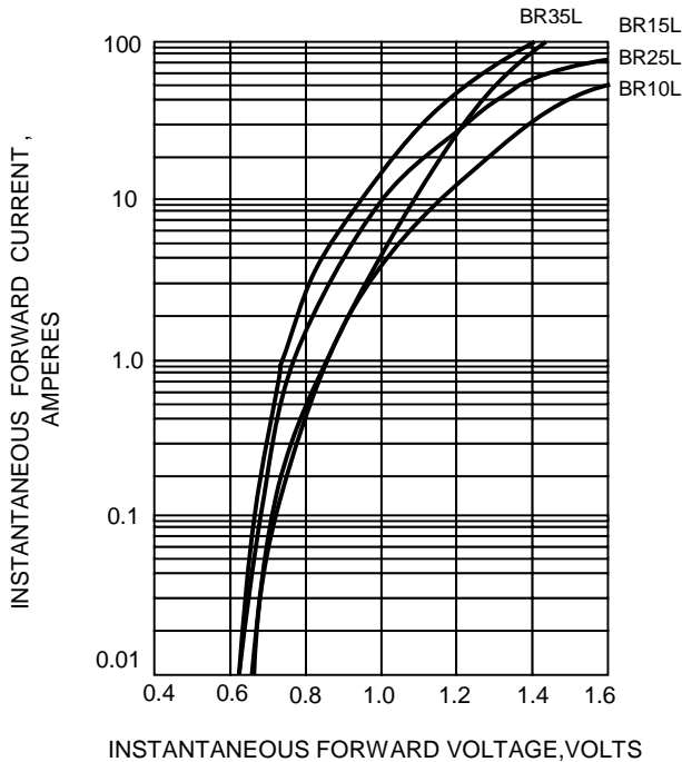
FIG.3-TYPICAL FORWARD CHARACTERISTICS
