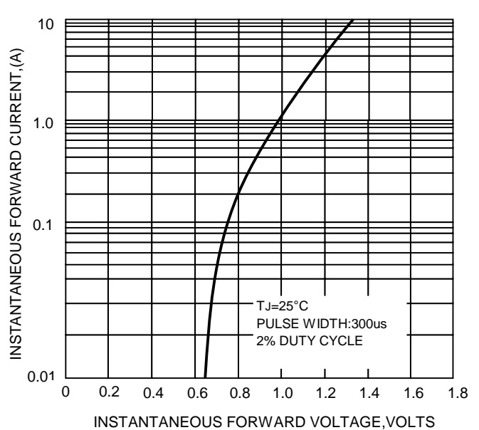
FIG.4-TYPICAL FORWARD CHARACTERISTICS
