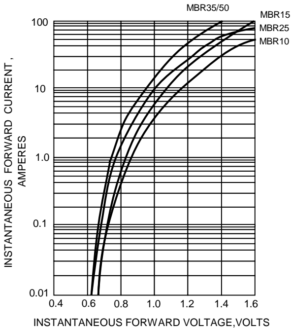
FIG.4-TYPICAL FORWARD CHARACTERISTICS
